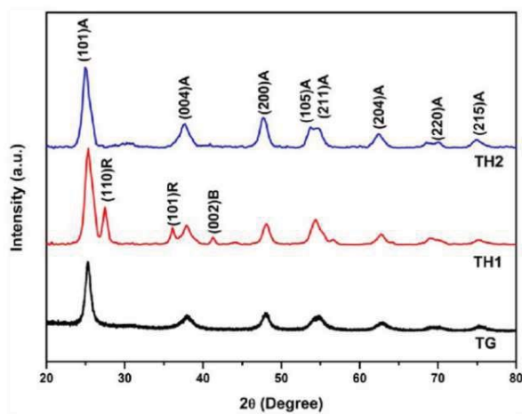
Fig. 3: XRD pattern of hydrothermally synthesized TiO 2 nanoparticles
